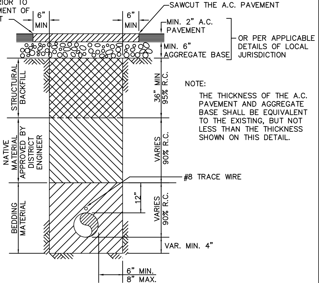
TYPICAL TRENCH SECTION
