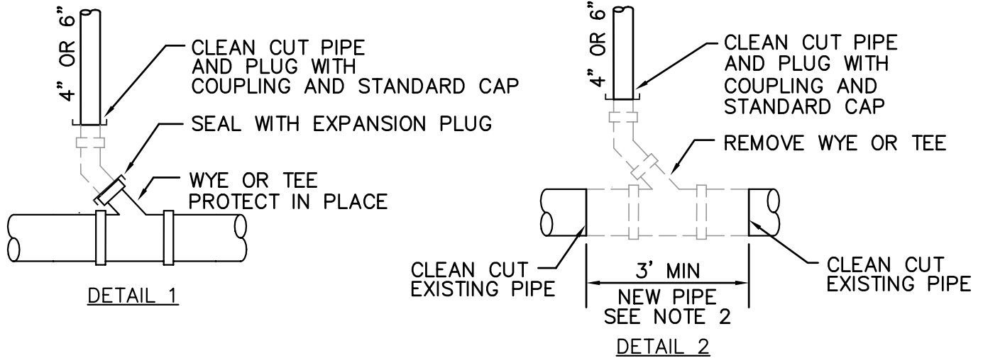
LATERAL DISCONNECTION AT MAIN SEWER (SEE NOTE 1)
