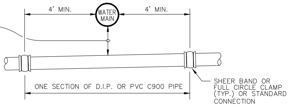
TYPICAL CROSSING UNDER WATER MAIN
